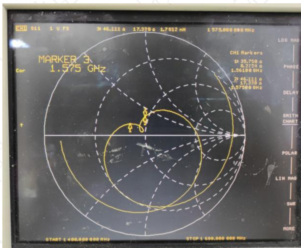
GPS Smith Chart (史密斯圆图)
