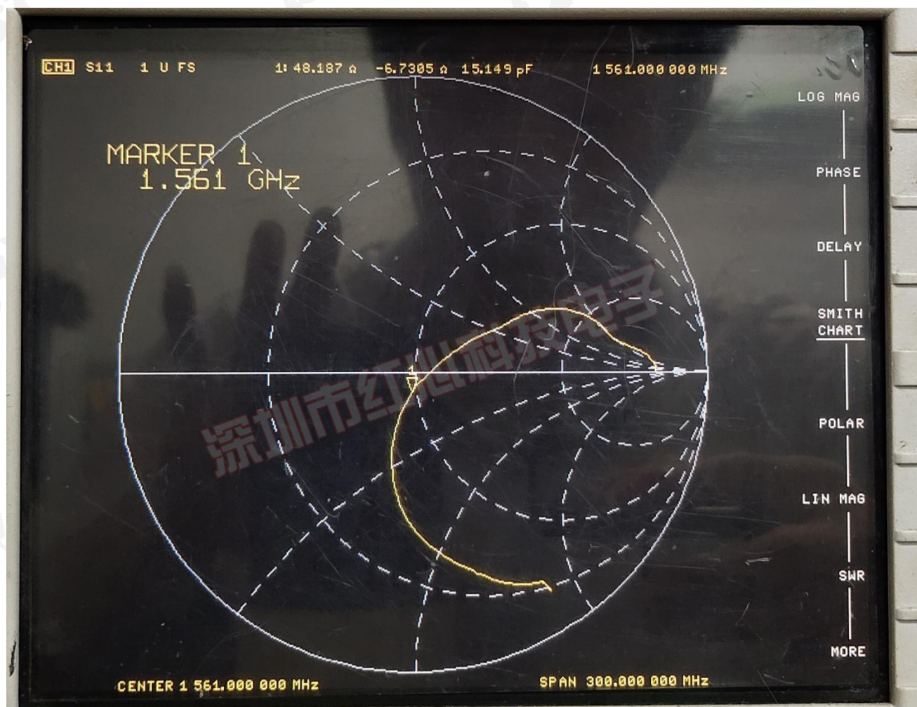
Smith Chart (史密斯圆图)
