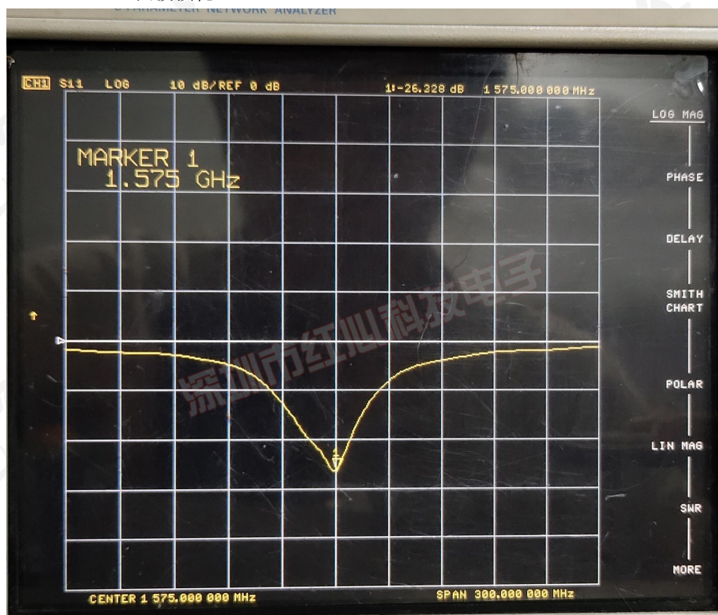
Return Loss (回波损耗)
