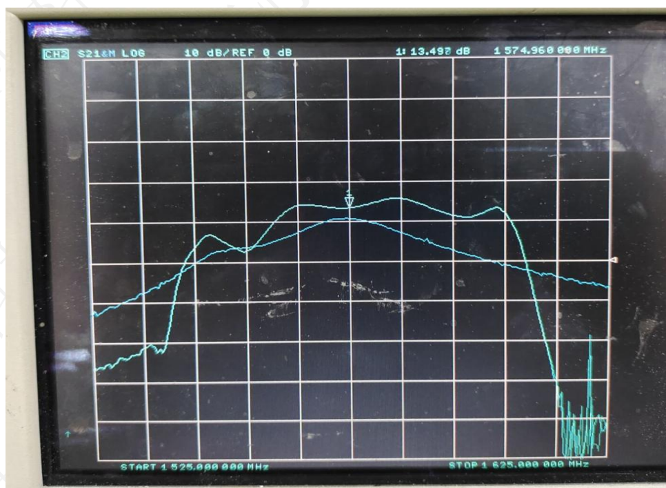
(Gain)增益图
