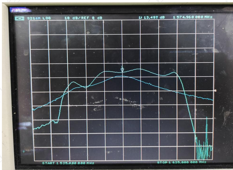
(Gain)增益图
