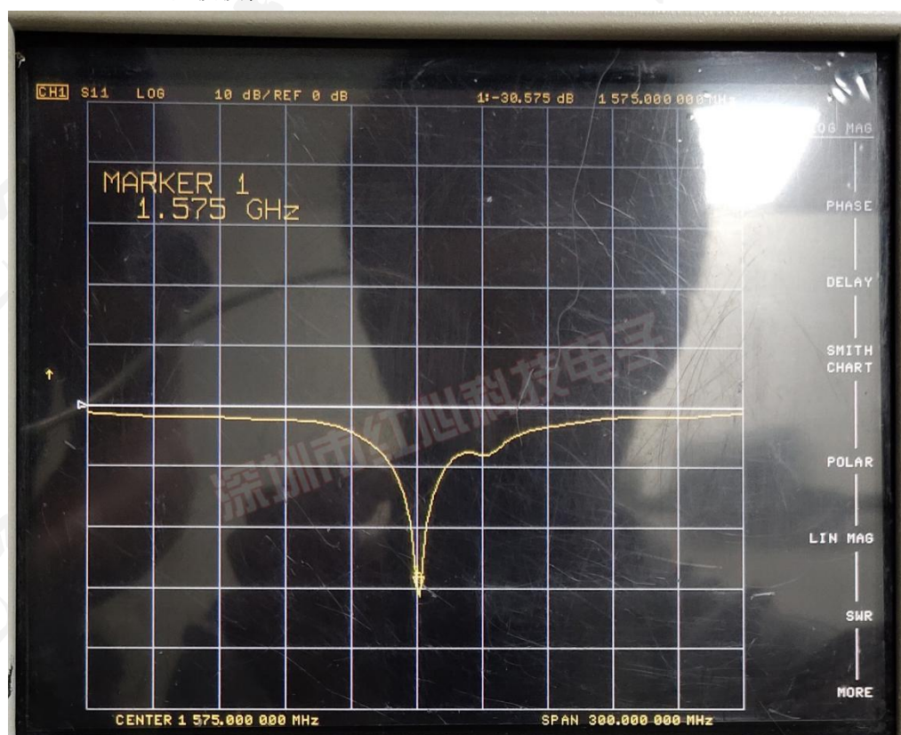
Return Loss (回波损耗)
