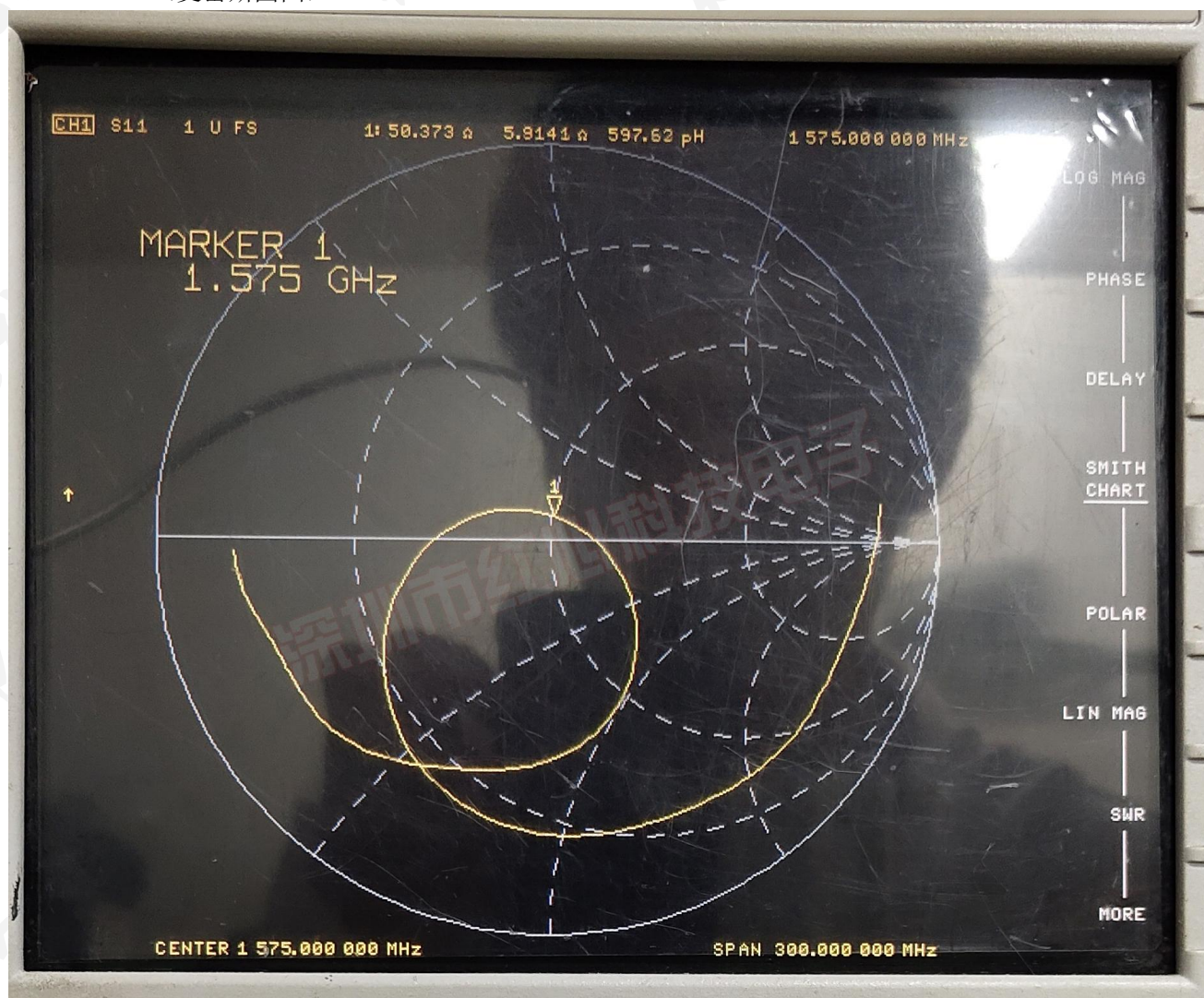
Smith Chart (史密斯圆图)
