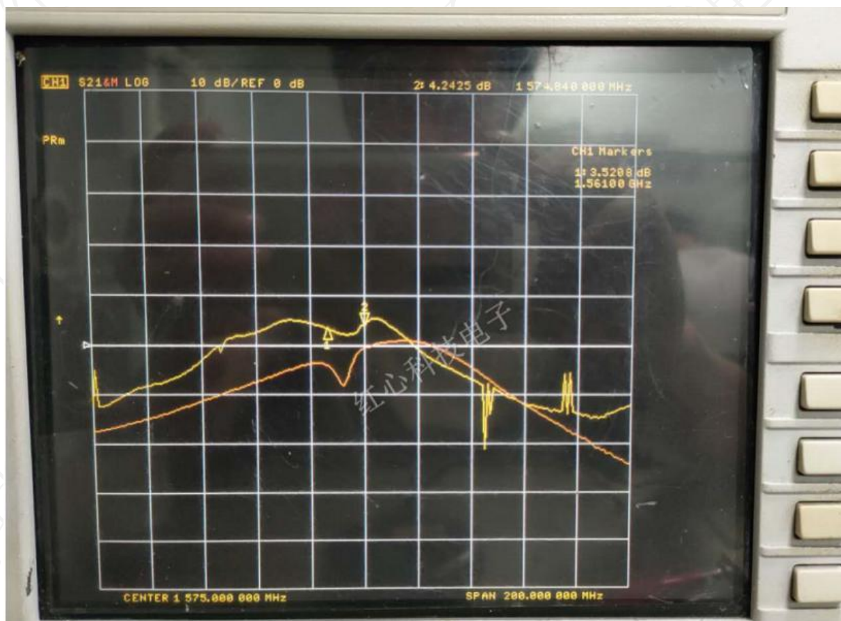
(Gain)增益图
