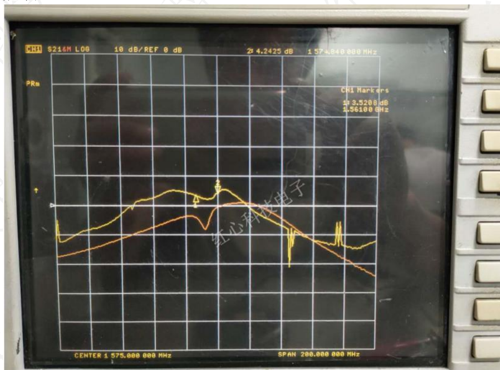
(Gain)增益图
