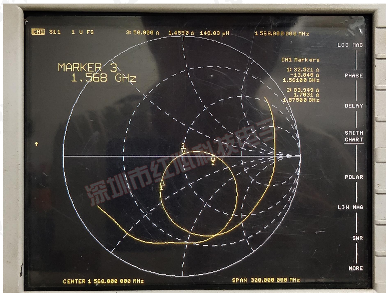
Smith Chart (史密斯圆图)
