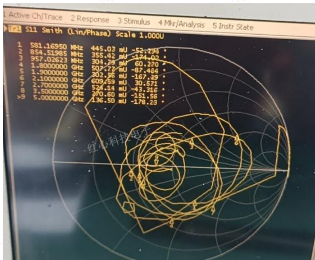
Smith Chart (史密斯圆图)
